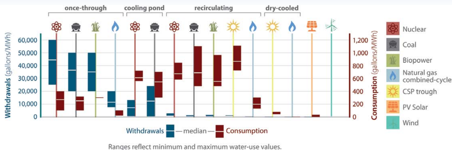
Figure 13. Water use by fuel and cooling technology
